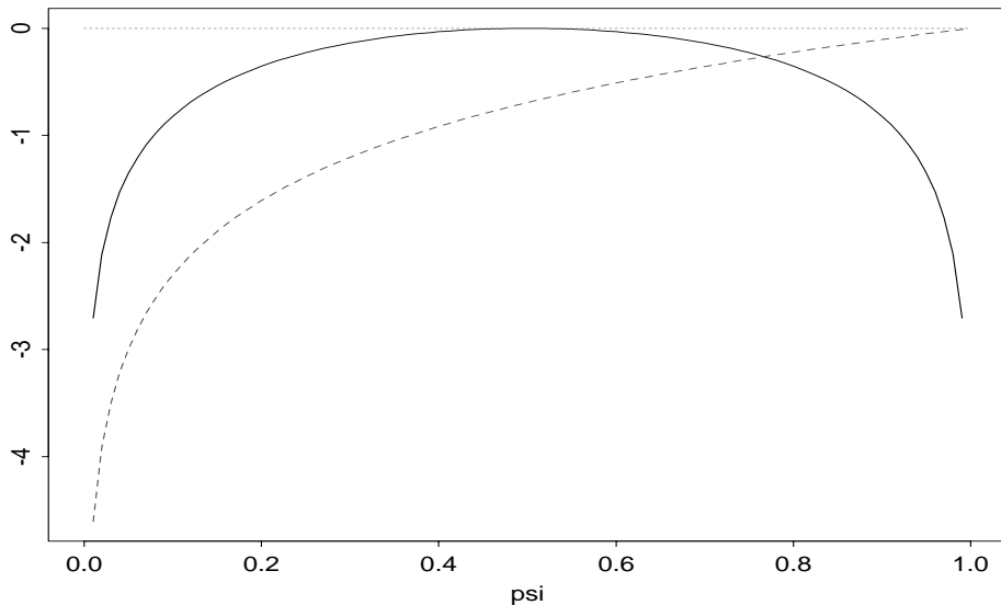
FIGURE 1: Three log-likelihoods consistent with a uniform confidence distribution over [0, 1] . ‘ Many likelihoods informed me of this before, which hung so tottering in the balance that I could neither believe nor misdoubt. ’ – SHAKESPEARE.
