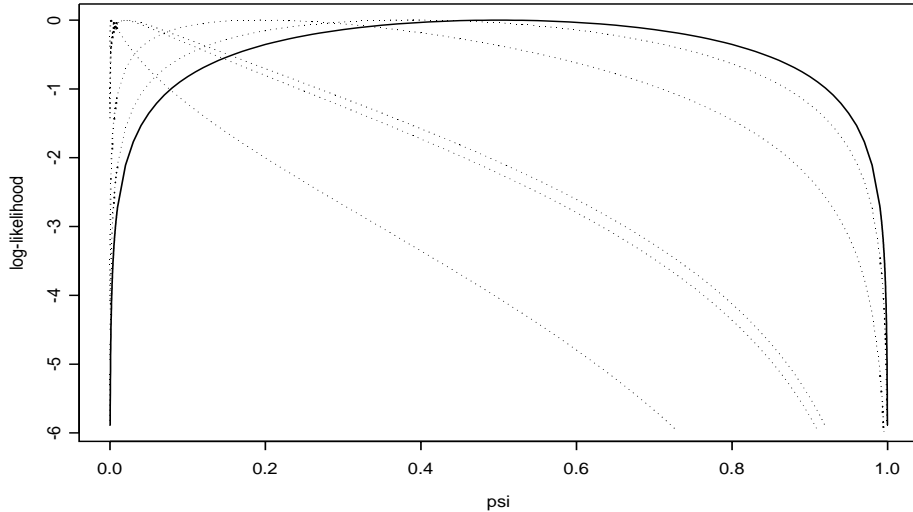
FIGURE 2: Normal-based log-likelihood related to a uniform confidence distribution over (0, 1) (solid line), along with five replicated bootstrap log-likelihoods (dotted).
