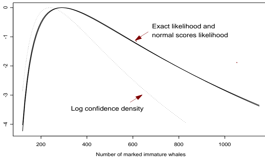
FIGURE 5: The exact likelihood is shown together with the normal scores likelihood, for the number of marked immature whales; these curves are almost identical. Also shown is the log-confidence density (dotted).
