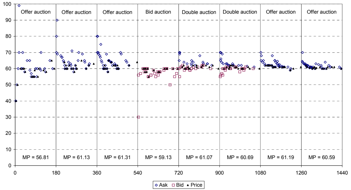
Figure 8. Asks, bids and prices, session AV1
